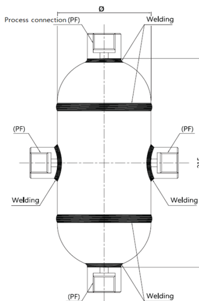
Mechanical accessories, series MA.93
