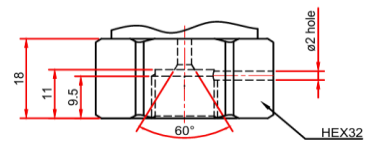
9/16-18 UNF Seal cone BOSS SAE J514
