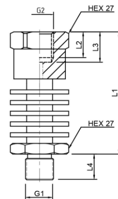
cooling device. product code AC44
