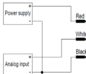
3-wire / voltage
